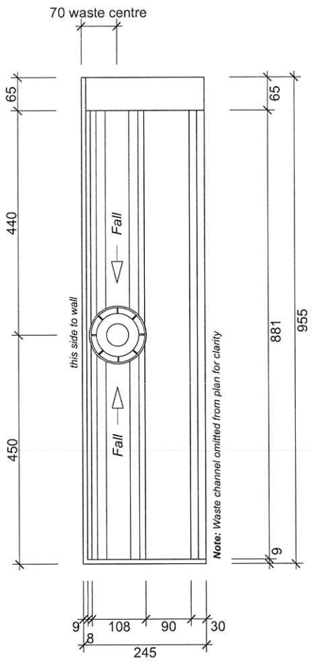
Floor Plan MB4 - 2-Wall Back Channel Drain & Satin Anodised Aluminium Tile Over Drain Cover 250x960 MB4-900-Plan
